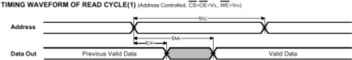
FIGURE 2. TIMING WAVEFORM OF READ CYCLE(1)
